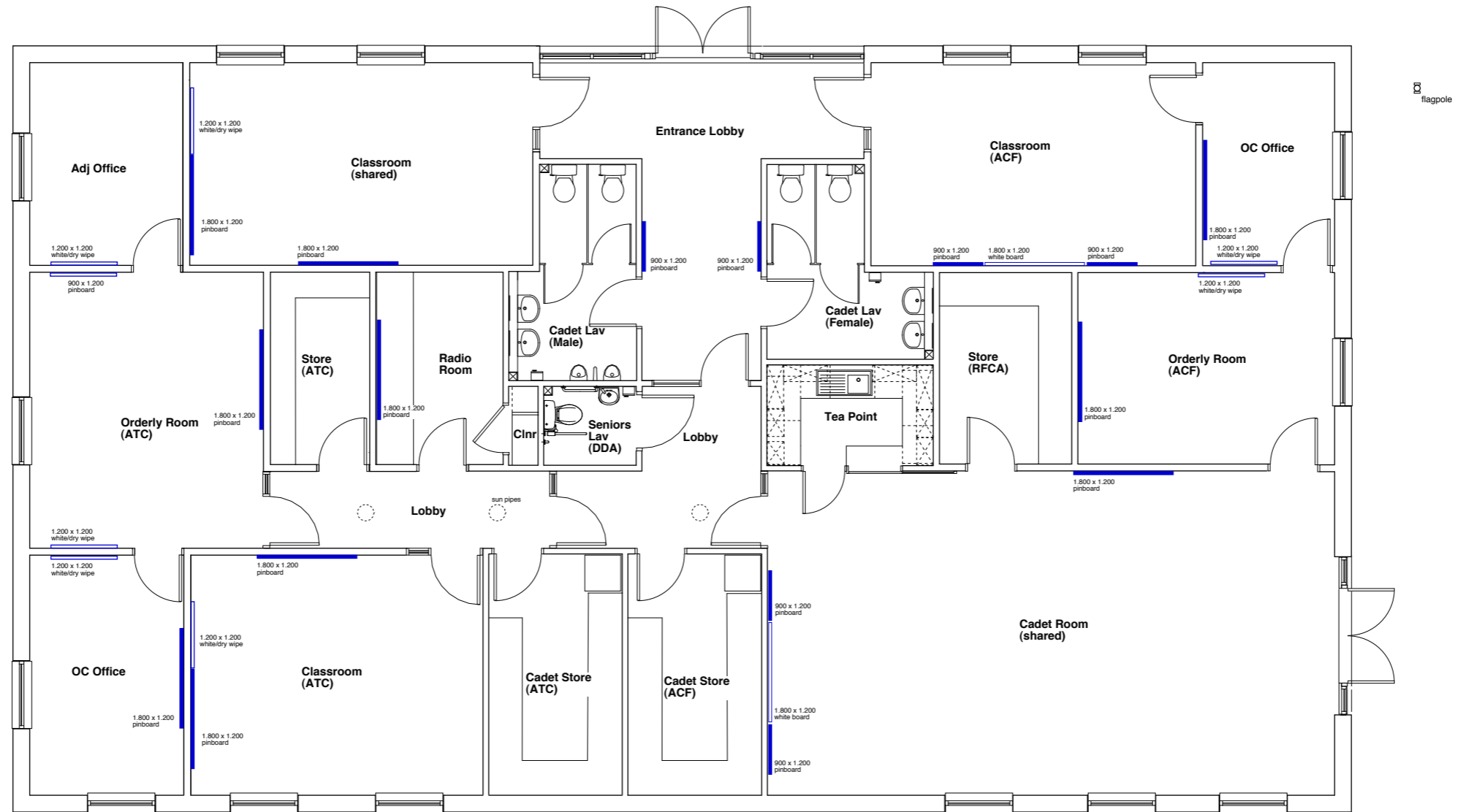
Ground Floor Plan 320 Sq M (nom. gross internal)
